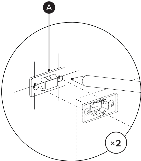
Mark on wall where second pair of brackets should be placed.
